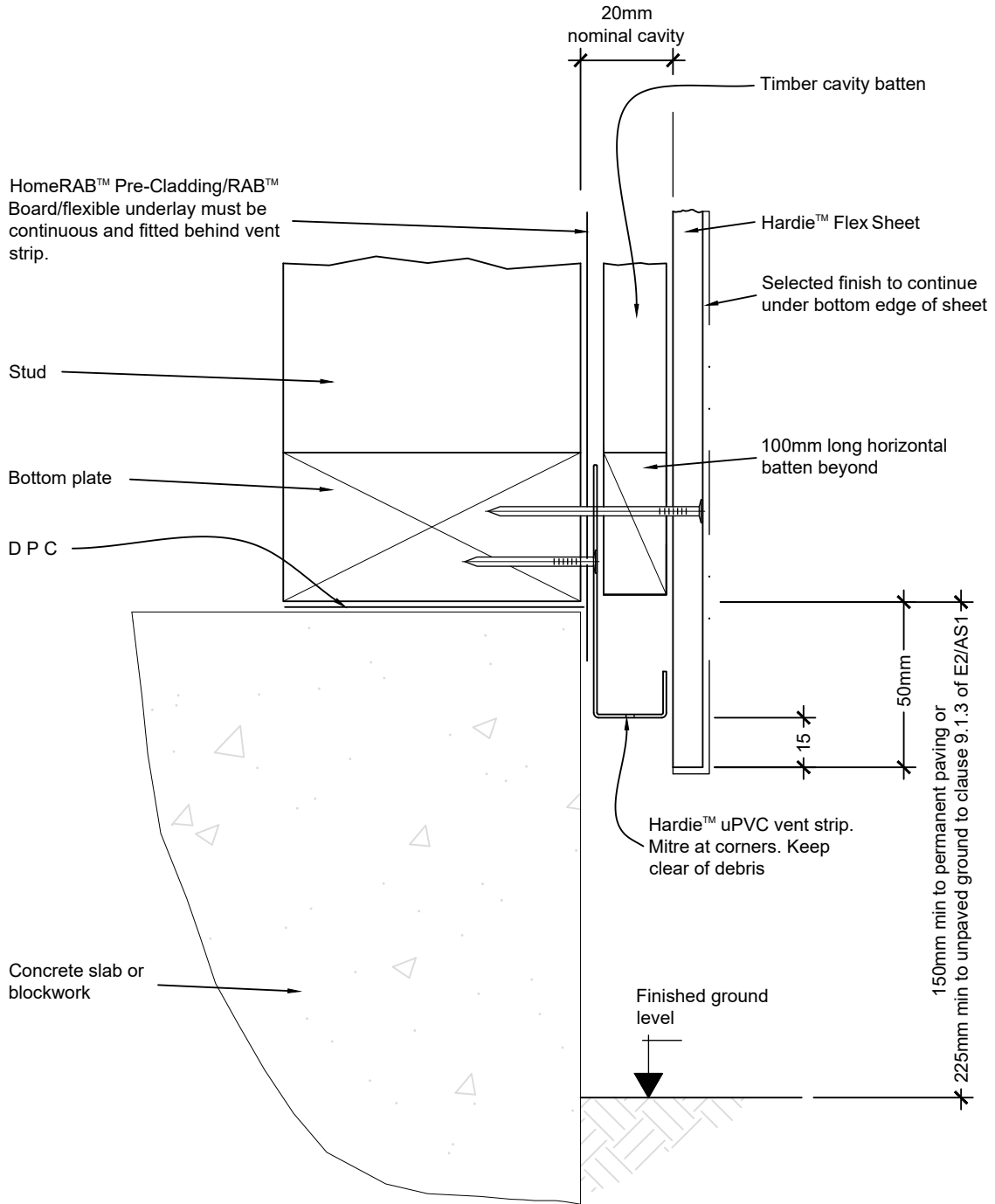
Foundation Detail
